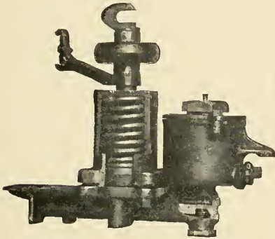
Fig. 69. Westinghouse Unit Switch Cylinder and Magnet Valve
